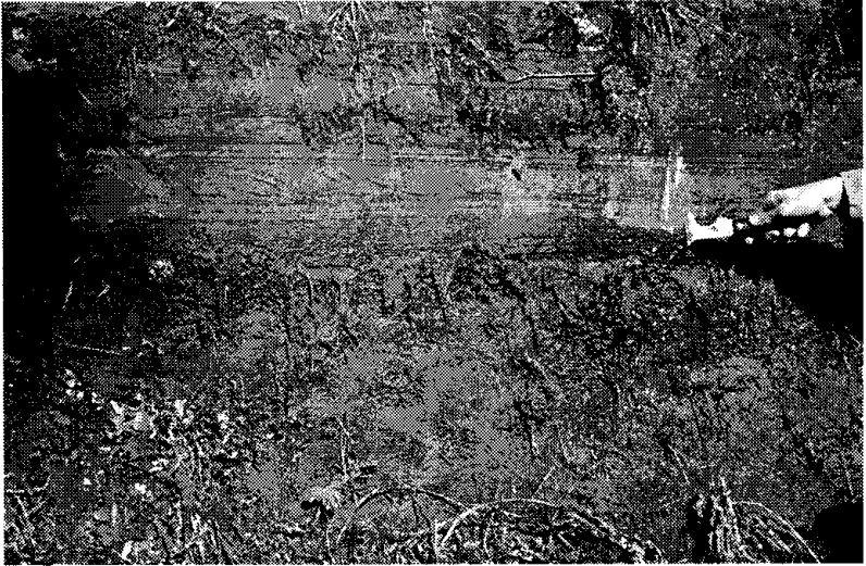
Figure 3 Soft sediment deformation structures in Unit 1.
