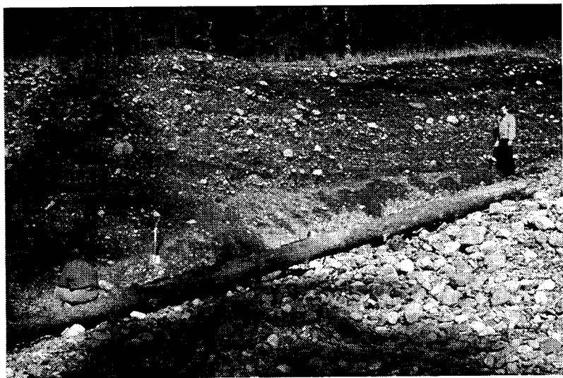
Figure 5 Cross-bedded sands and gravels in Unit 3.
